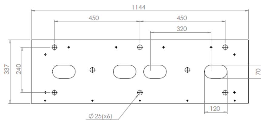
Measurements of foot plate
